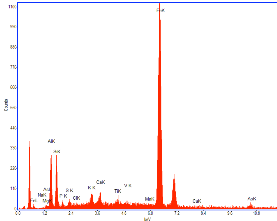
FIGURE 6. EDS spectrum of iron oxide coating showing detectable arsenic (AsK) in the lower right part of the image (analysis taken at 30kV, high vacuum, uncoated sample).
